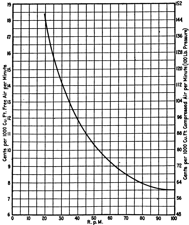
FIG. 122.—Test results of compressor plant No. 2.
